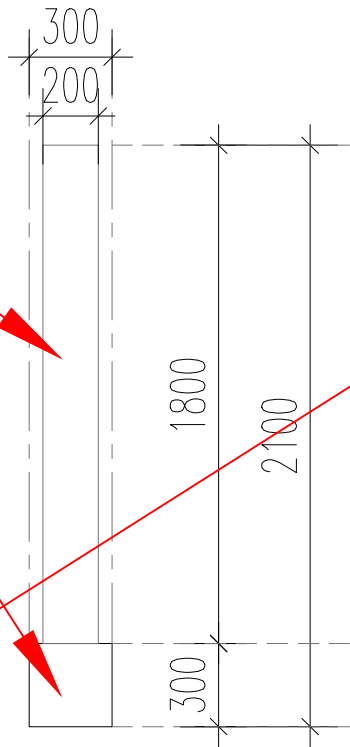
ADVERTISING BOARD SIDE ELEVATION
