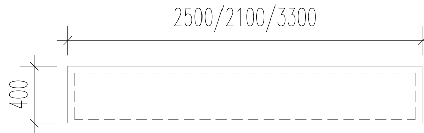
PLANTER BOX - SEATING AREA 01& 02 FRONT & REAR ELEVATION
