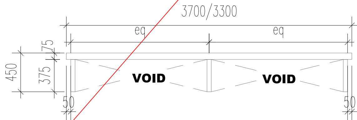
BENCH - SEATING AREA 01& 02 FRONT ELEVATION
